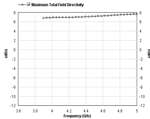
Fig 26: Directivity Graph (Showing a Directivity of 7.58 at 4.96 GHz) for Slotted Rectangular Patch Antenna
