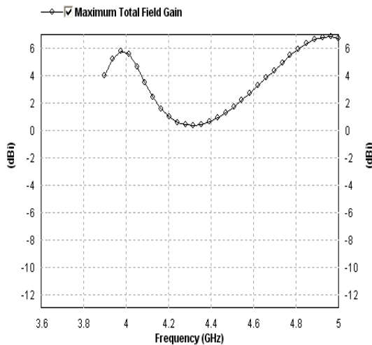
Fig 24: Field Gain (6.77dBi for the Second Band) of Slotted Microstrip Rectangular Patch Antenna
